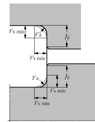
Fig. 15.8 Bearing mounting with spacer
